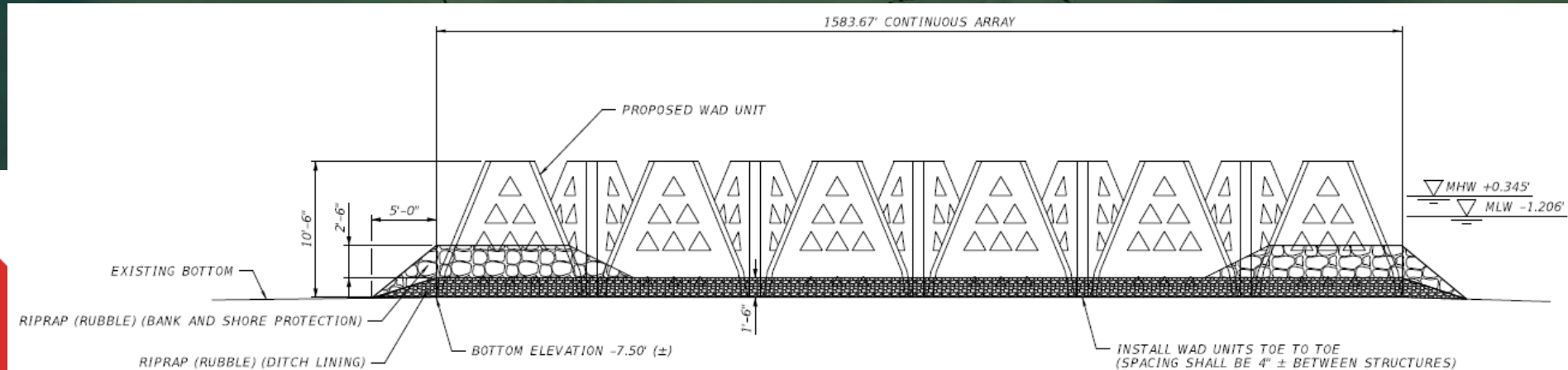
WAD PROFILE SECTION
